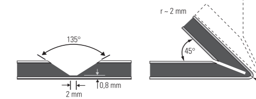
135° V-groove for folds up to 135°
