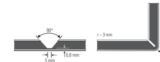
90° V-groove for folds up to 90°
